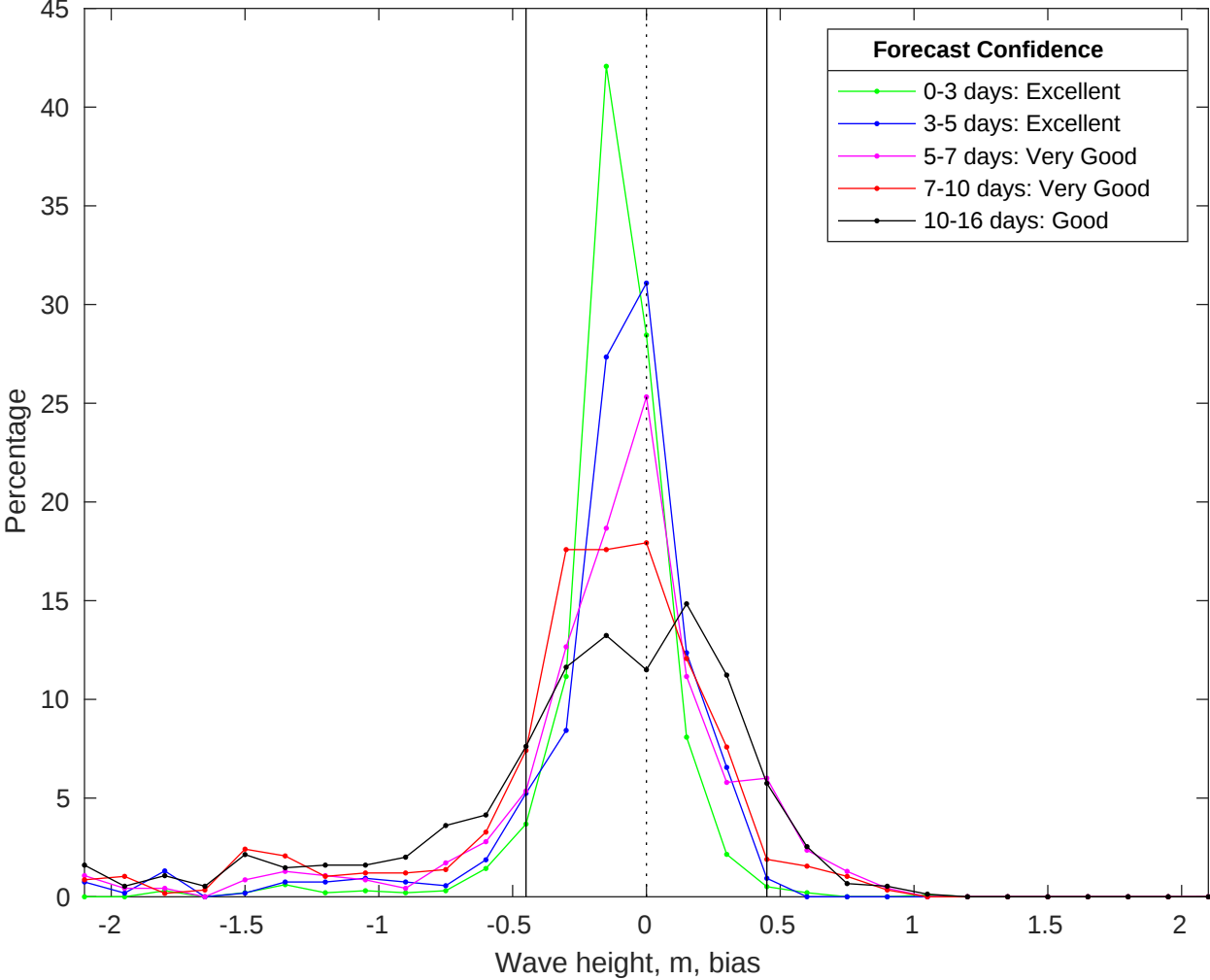
NDBC 41013 vs GFS Waves Bias Histogram: 11-Jul-2025
