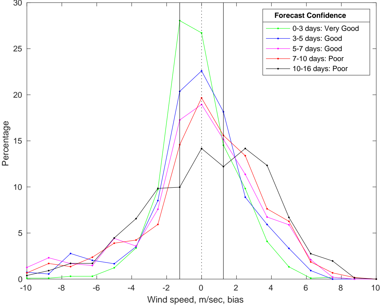
NDBC 41013 vs GFS Winds Bias Histogram: 11-Jul-2025
