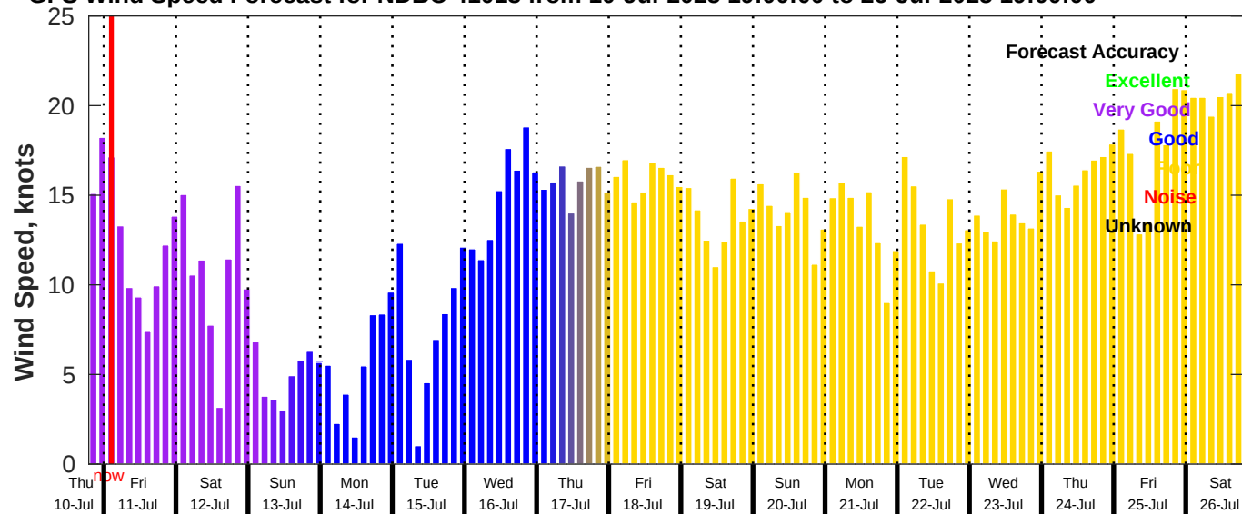
GFS Wind Speed Forecast for NDBC 41013 from 10-Jul-2025 19:00:00 to 26-Jul-2025 19:00:00
