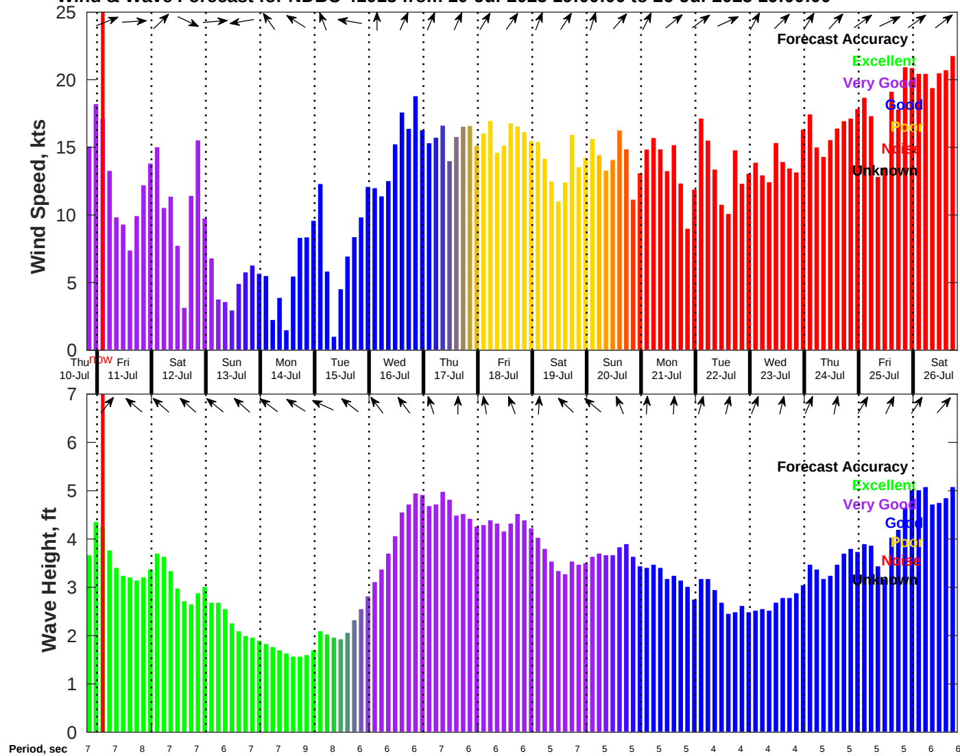
Wind & Wave Forecast for NDBC 41013 from 10-Jul-2025 19:00:00 to 26-Jul-2025 19:00:00
