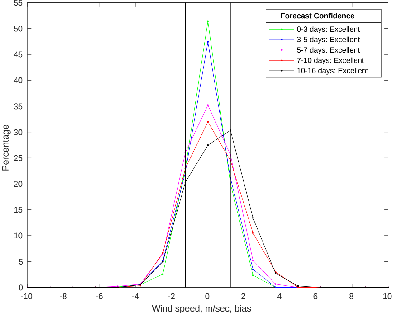
NDBC 41040 vs GFS Winds Bias Histogram: 11-Jul-2025
