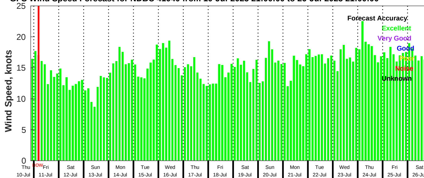
GFS Wind Speed Forecast for NDBC 41040 from 10-Jul-2025 21:00:00 to 26-Jul-2025 21:00:00
