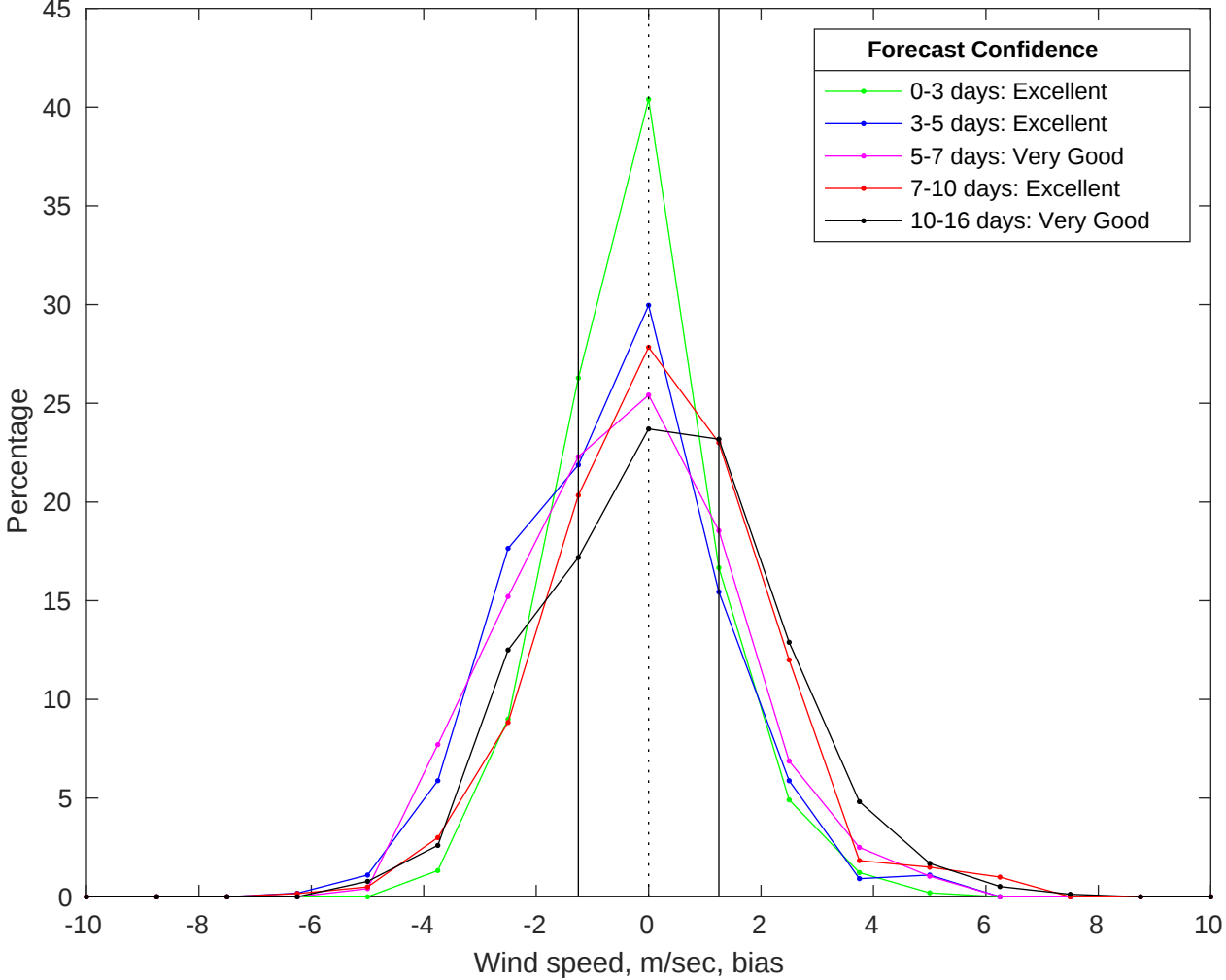
NDBC 42019 vs GFS Winds Bias Histogram: 11-Jul-2025
