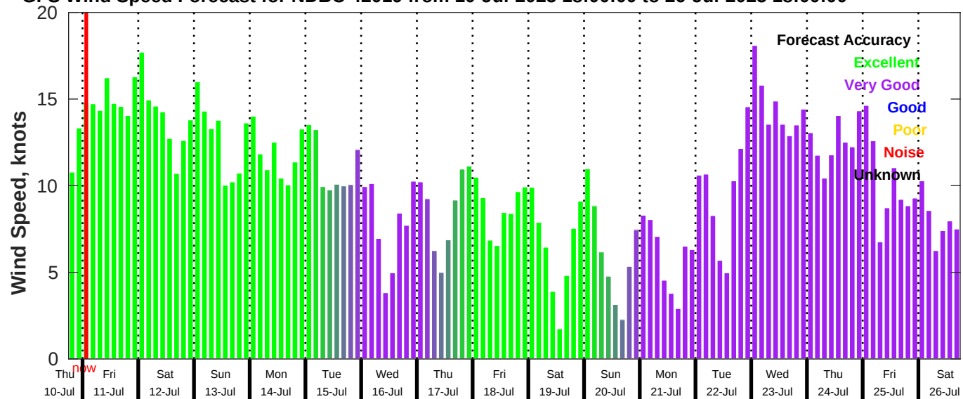
GFS Wind Speed Forecast for NDBC 42019 from 10-Jul-2025 18:00:00 to 26-Jul-2025 18:00:00
