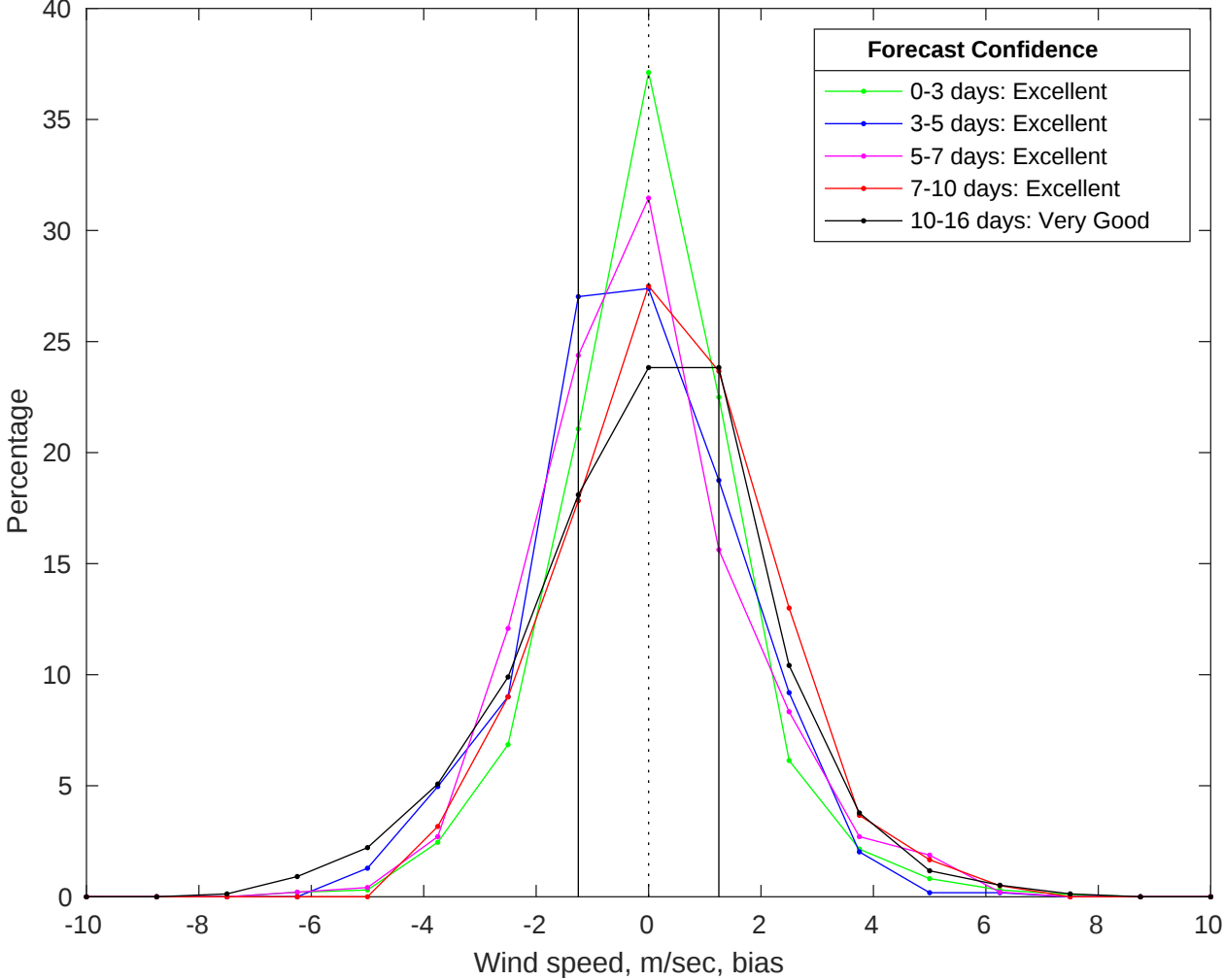
NDBC 42020 vs GFS Winds Bias Histogram: 11-Jul-2025
