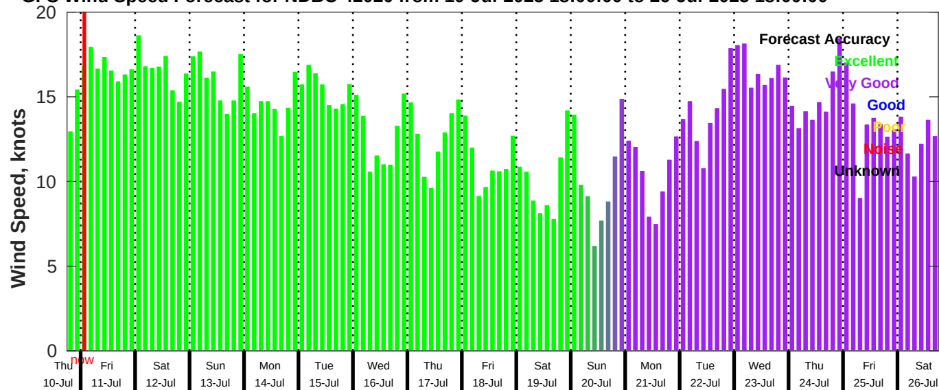
GFS Wind Speed Forecast for NDBC 42020 from 10-Jul-2025 18:00:00 to 26-Jul-2025 18:00:00
