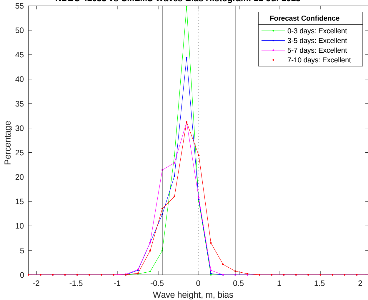
NDBC 42035 vs CMEMS Waves Bias Histogram: 11-Jul-2025
