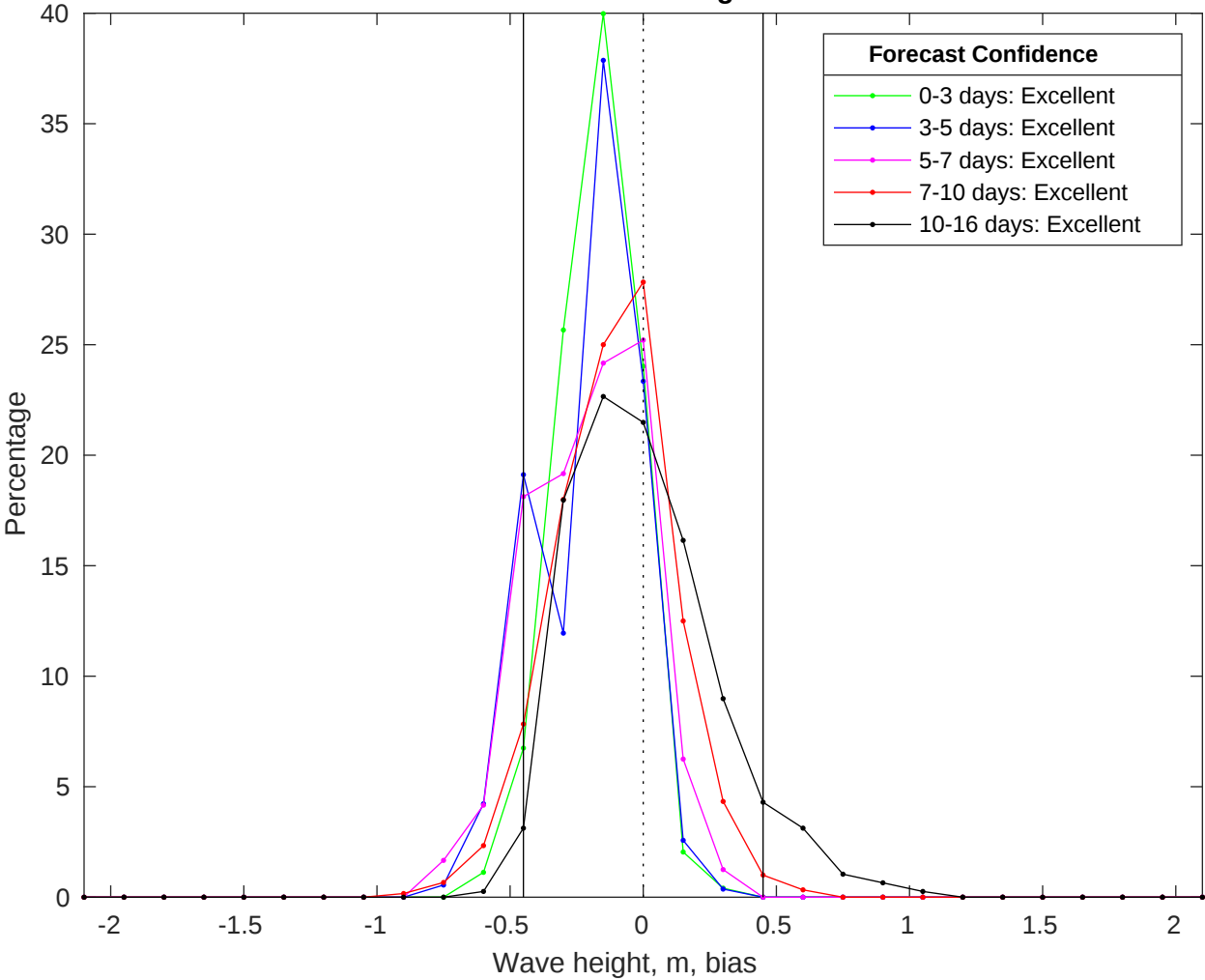
NDBC 42035 vs GFS Waves Bias Histogram: 11-Jul-2025
