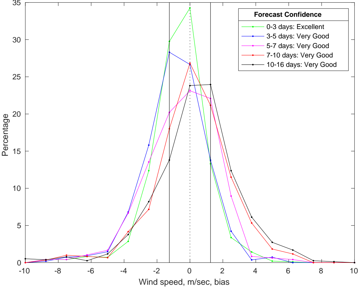
NDBC 42035 vs GFS Winds Bias Histogram: 11-Jul-2025
