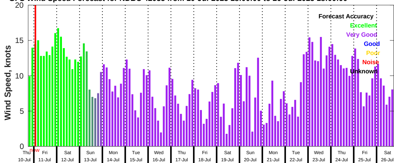
GFS Wind Speed Forecast for NDBC 42035 from 10-Jul-2025 18:00:00 to 26-Jul-2025 18:00:00
