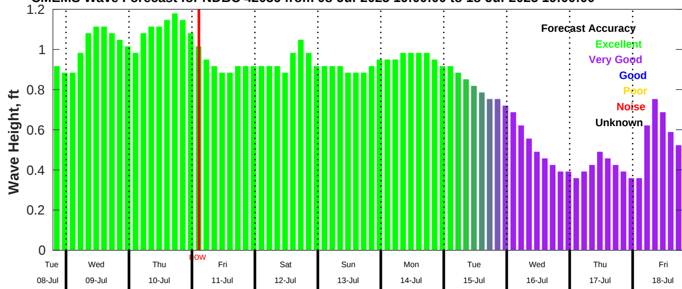
CMEMS Wave Forecast for NDBC 42036 from 08-Jul-2025 19:00:00 to 18-Jul-2025 19:00:00
