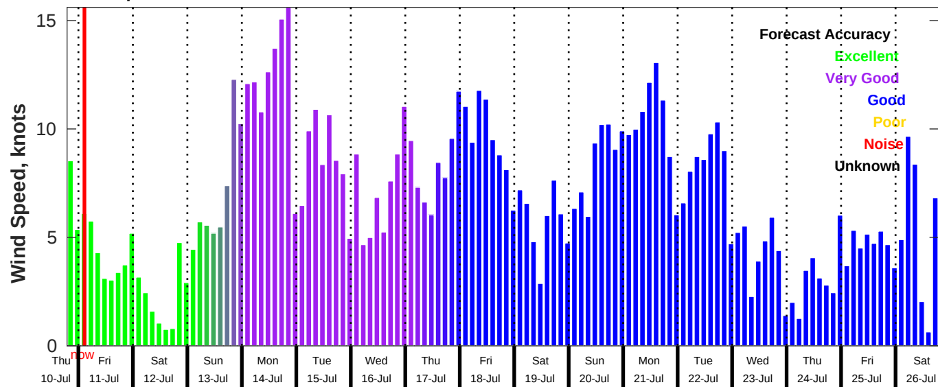
GFS Wind Speed Forecast for NDBC 42036 from 10-Jul-2025 19:00:00 to 26-Jul-2025 19:00:00
