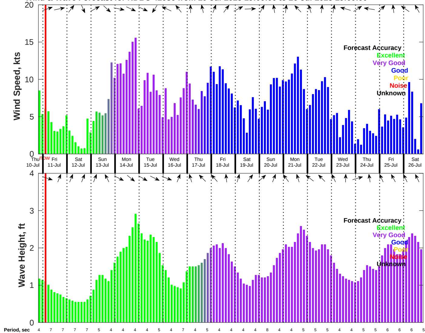
Wind & Wave Forecast for NDBC 42036 from 10-Jul-2025 19:00:00 to 26-Jul-2025 19:00:00
