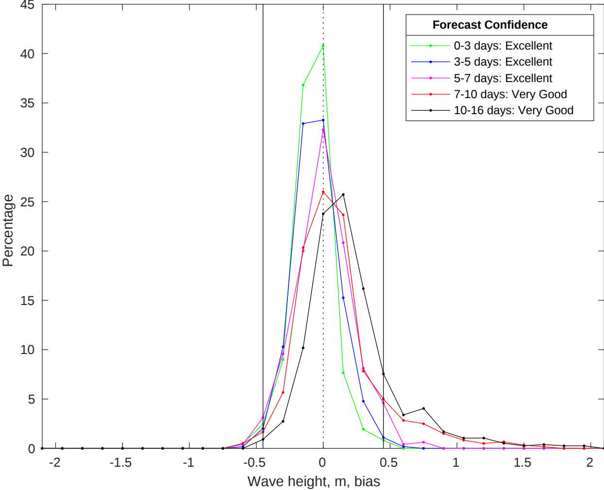
NDBC 42040 vs GFS Waves Bias Histogram: 11-Jul-2025
