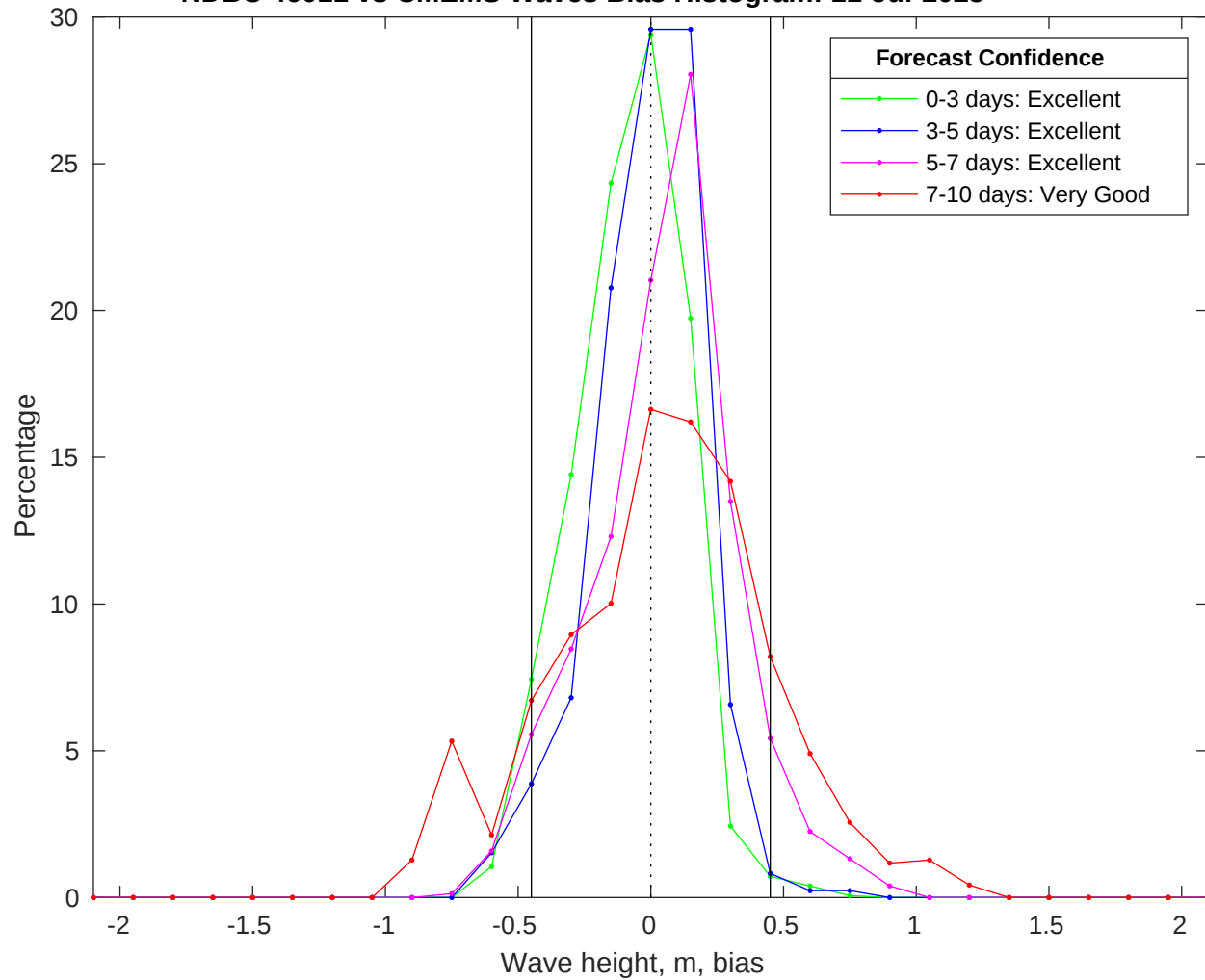
NDBC 46011 vs CMEMS Waves Bias Histogram: 11-Jul-2025
