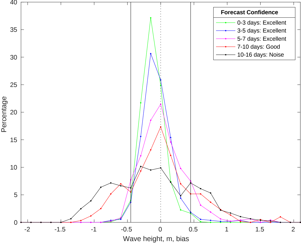
NDBC 46011 vs GFS Waves Bias Histogram: 11-Jul-2025
