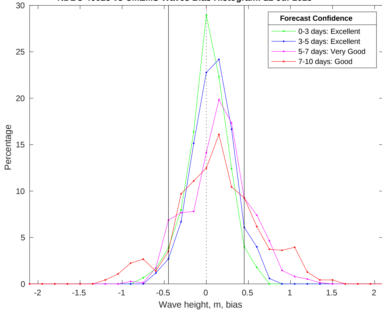
NDBC 46028 vs CMEMS Waves Bias Histogram: 11-Jul-2025
