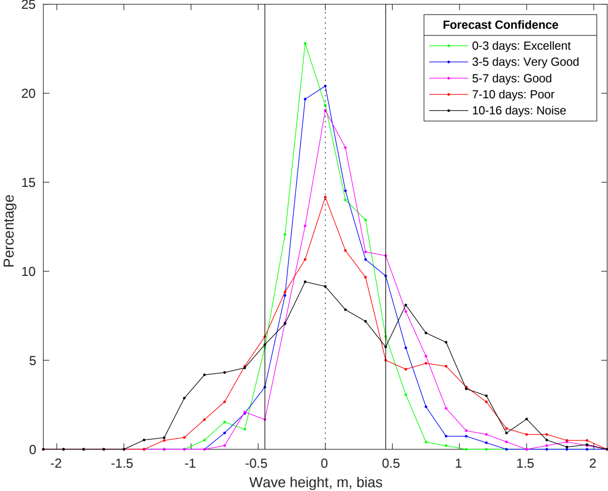
NDBC 46028 vs GFS Waves Bias Histogram: 11-Jul-2025
