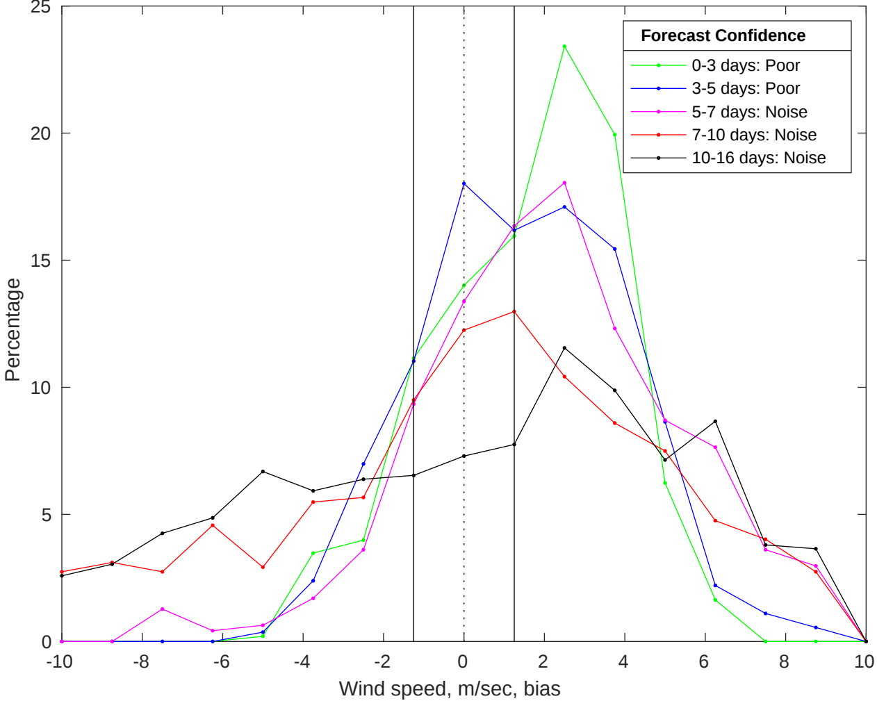
NDBC 46028 vs GFS Winds Bias Histogram: 11-Jul-2025
