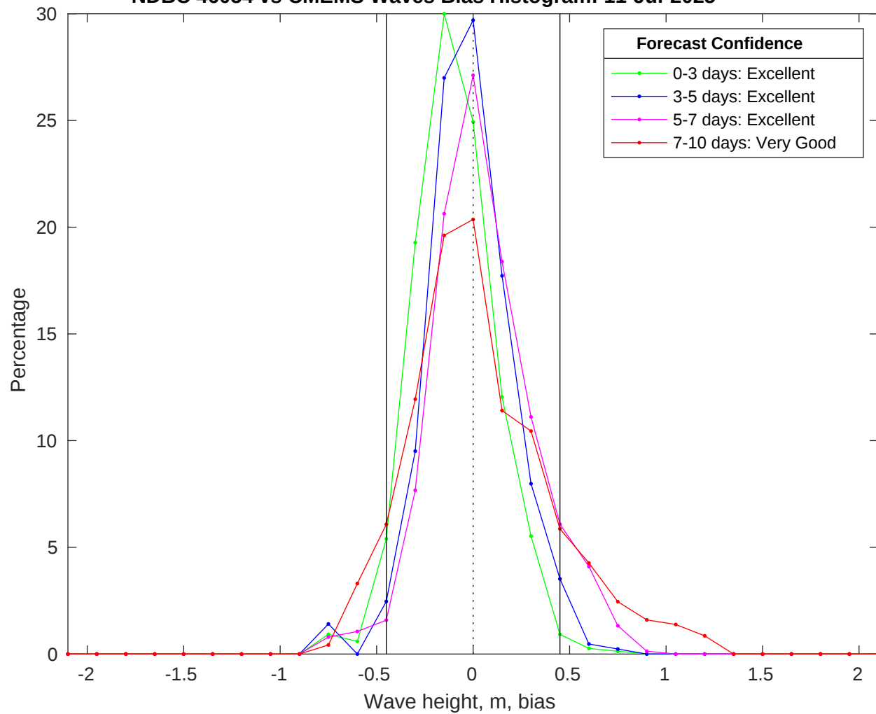
NDBC 46054 vs CMEMS Waves Bias Histogram: 11-Jul-2025
