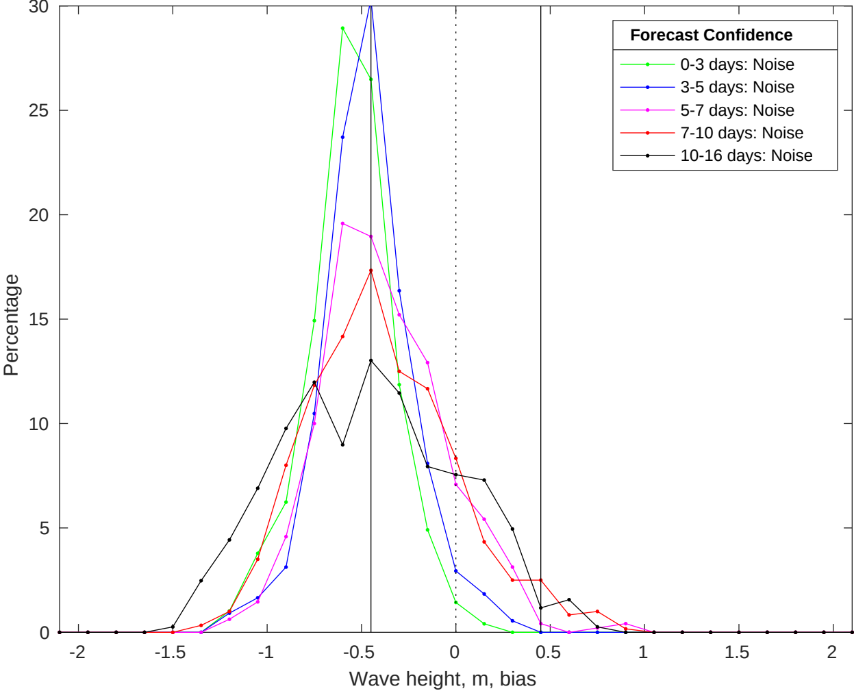
NDBC 46054 vs GFS Waves Bias Histogram: 11-Jul-2025
