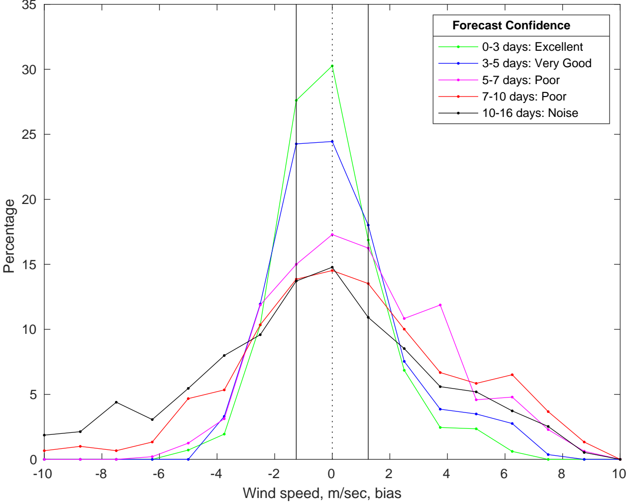
NDBC 46054 vs GFS Winds Bias Histogram: 11-Jul-2025
