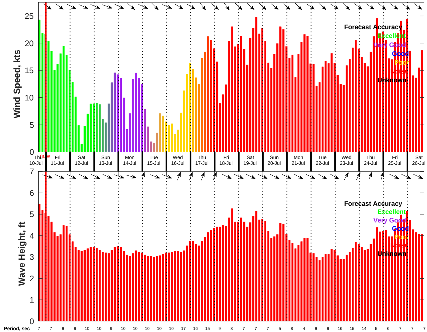
Wind & Wave Forecast for NDBC 46054 from 10-Jul-2025 16:00:00 to 26-Jul-2025 16:00:00
