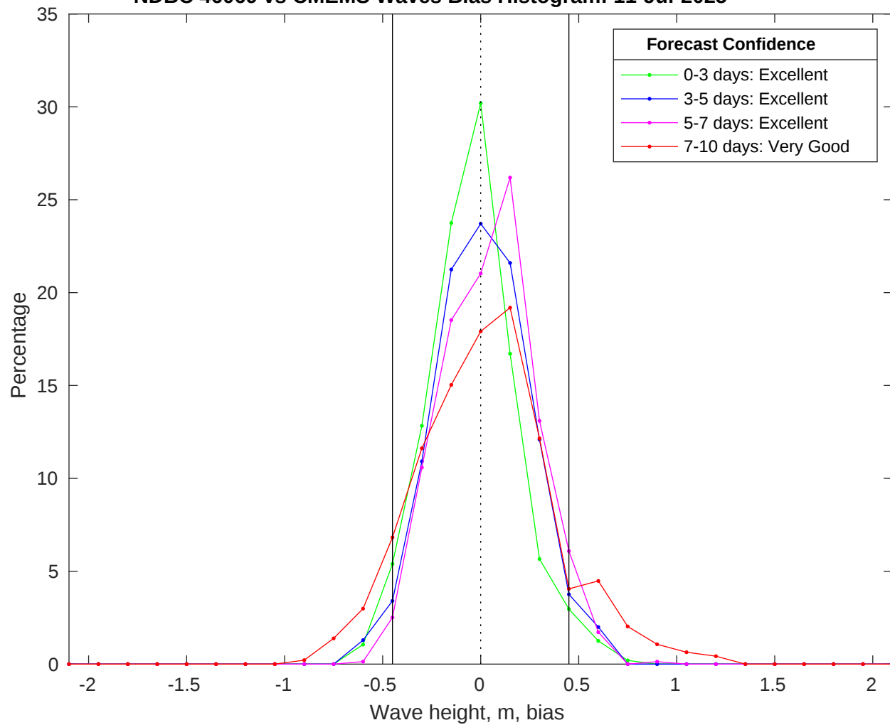
NDBC 46069 vs CMEMS Waves Bias Histogram: 11-Jul-2025
