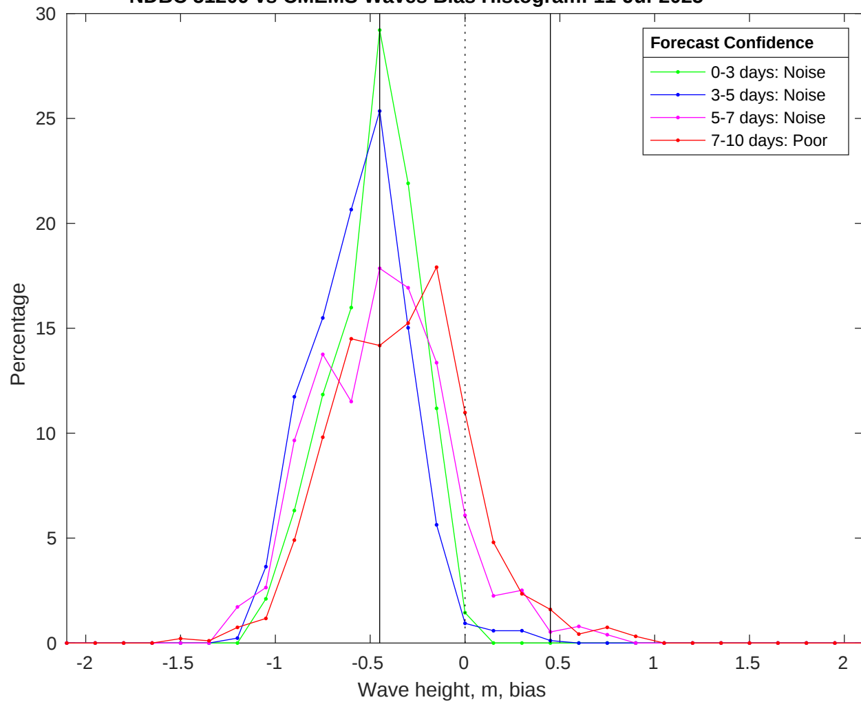
NDBC 51209 vs CMEMS Waves Bias Histogram: 11-Jul-2025
