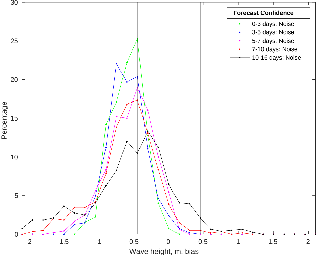
NDBC 51209 vs GFS Waves Bias Histogram: 11-Jul-2025
