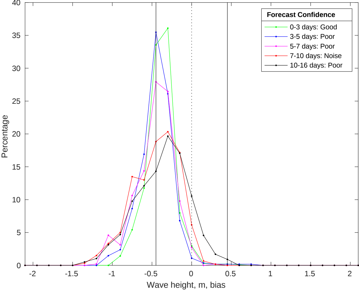
NDBC 52213 vs GFS Waves Bias Histogram: 11-Jul-2025
