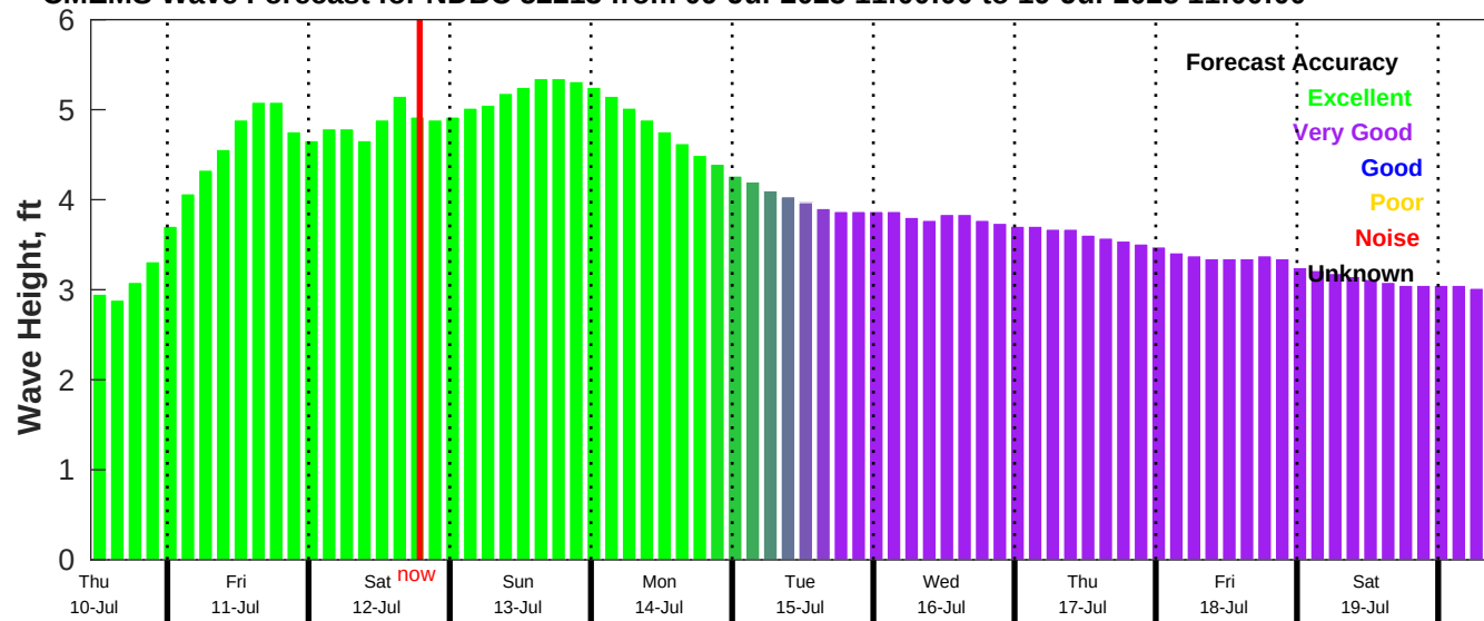
CMEMS Wave Forecast for NDBC 52213 from 09-Jul-2025 11:00:00 to 19-Jul-2025 11:00:00
