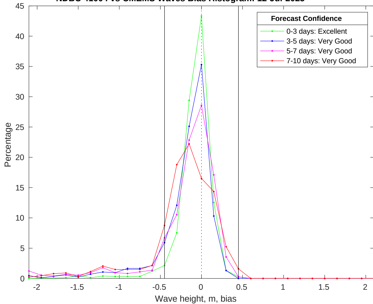
NDBC 41004 vs CMEMS Waves Bias Histogram: 12-Jul-2025
