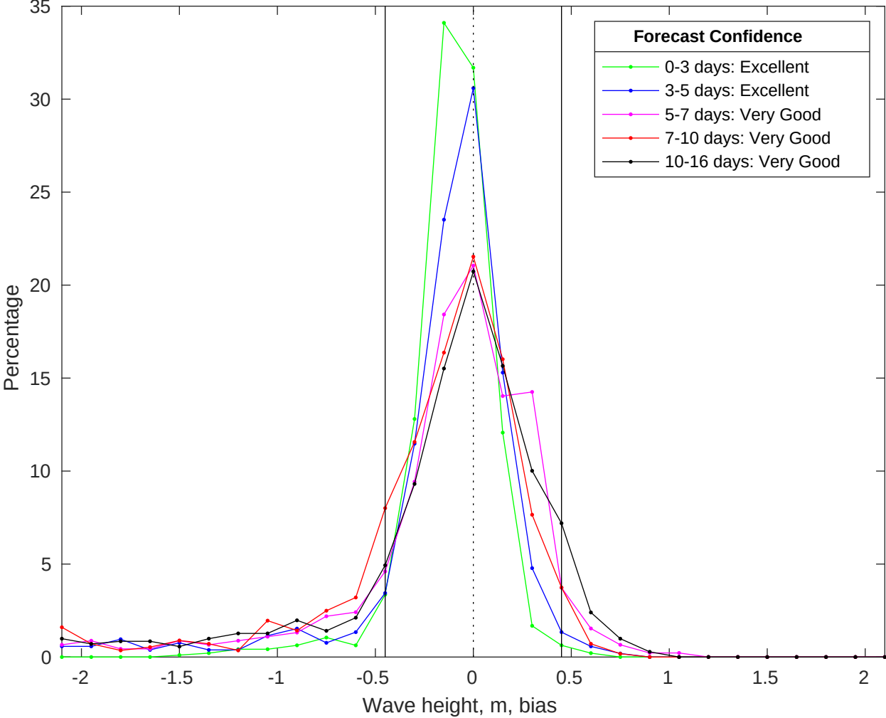
NDBC 41004 vs GFS Waves Bias Histogram: 12-Jul-2025
