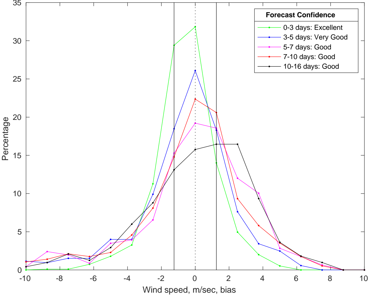
NDBC 41004 vs GFS Winds Bias Histogram: 12-Jul-2025
