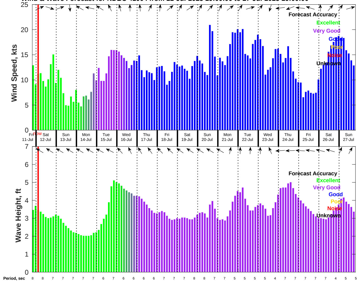
Wind & Wave Forecast for NDBC 41004 from 11-Jul-2025 19:00:00 to 27-Jul-2025 19:00:00
