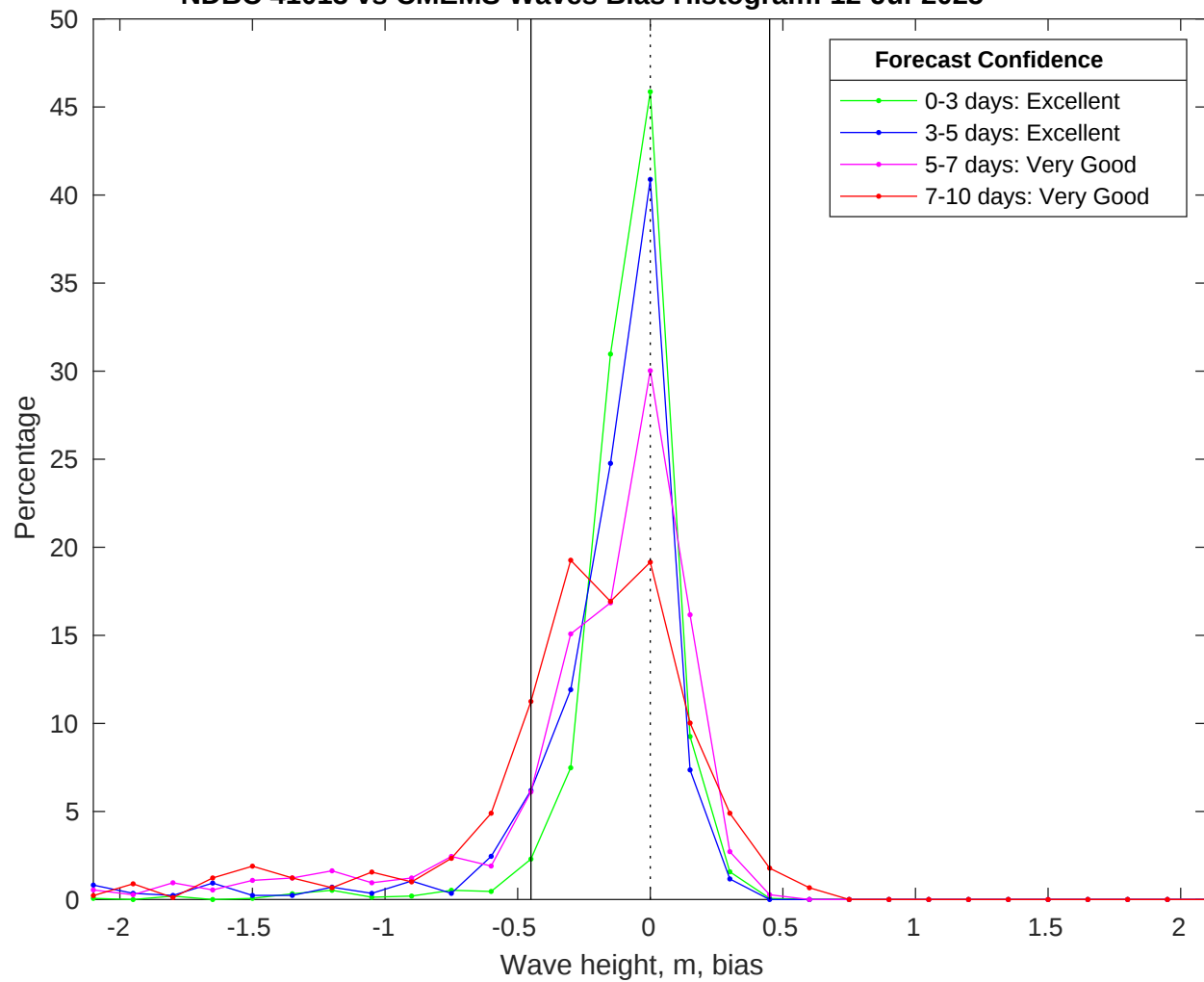
NDBC 41013 vs CMEMS Waves Bias Histogram: 12-Jul-2025
