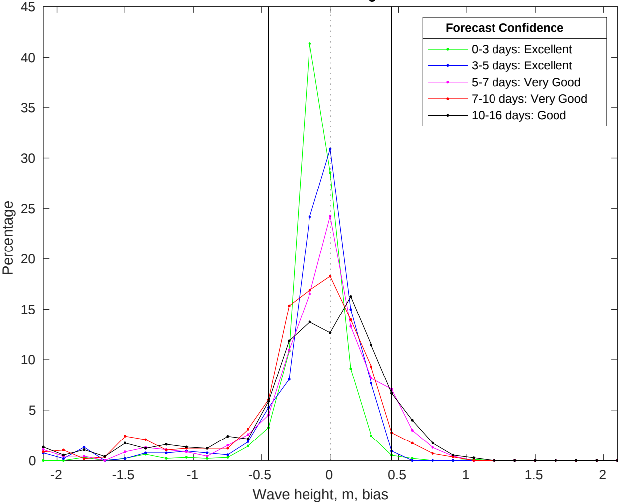
NDBC 41013 vs GFS Waves Bias Histogram: 12-Jul-2025
