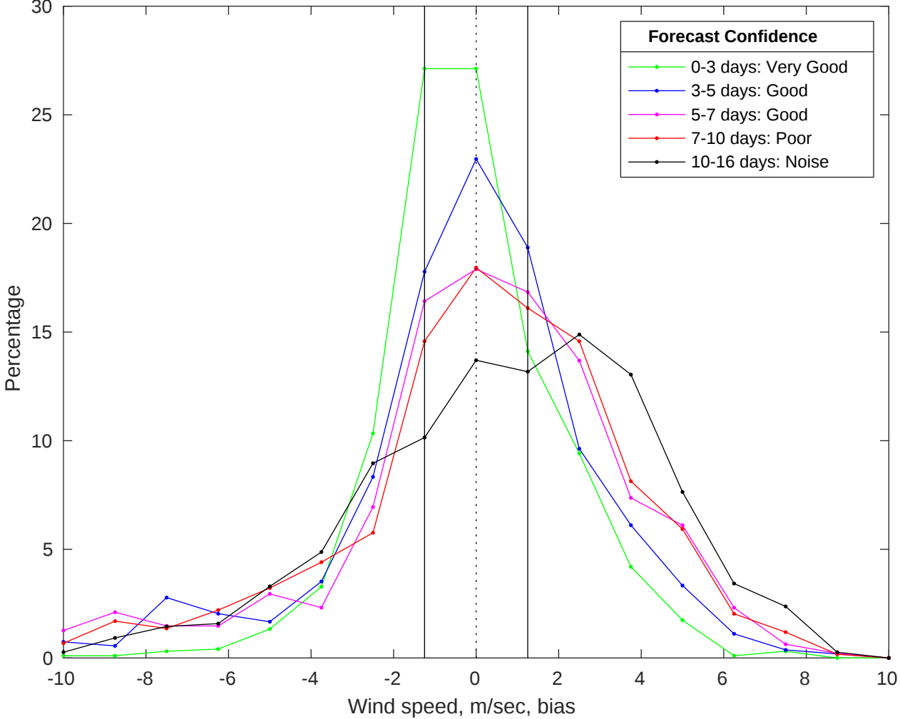
NDBC 41013 vs GFS Winds Bias Histogram: 12-Jul-2025
