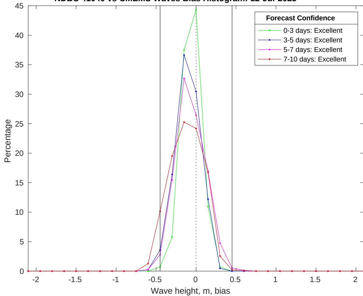
NDBC 41040 vs CMEMS Waves Bias Histogram: 12-Jul-2025
