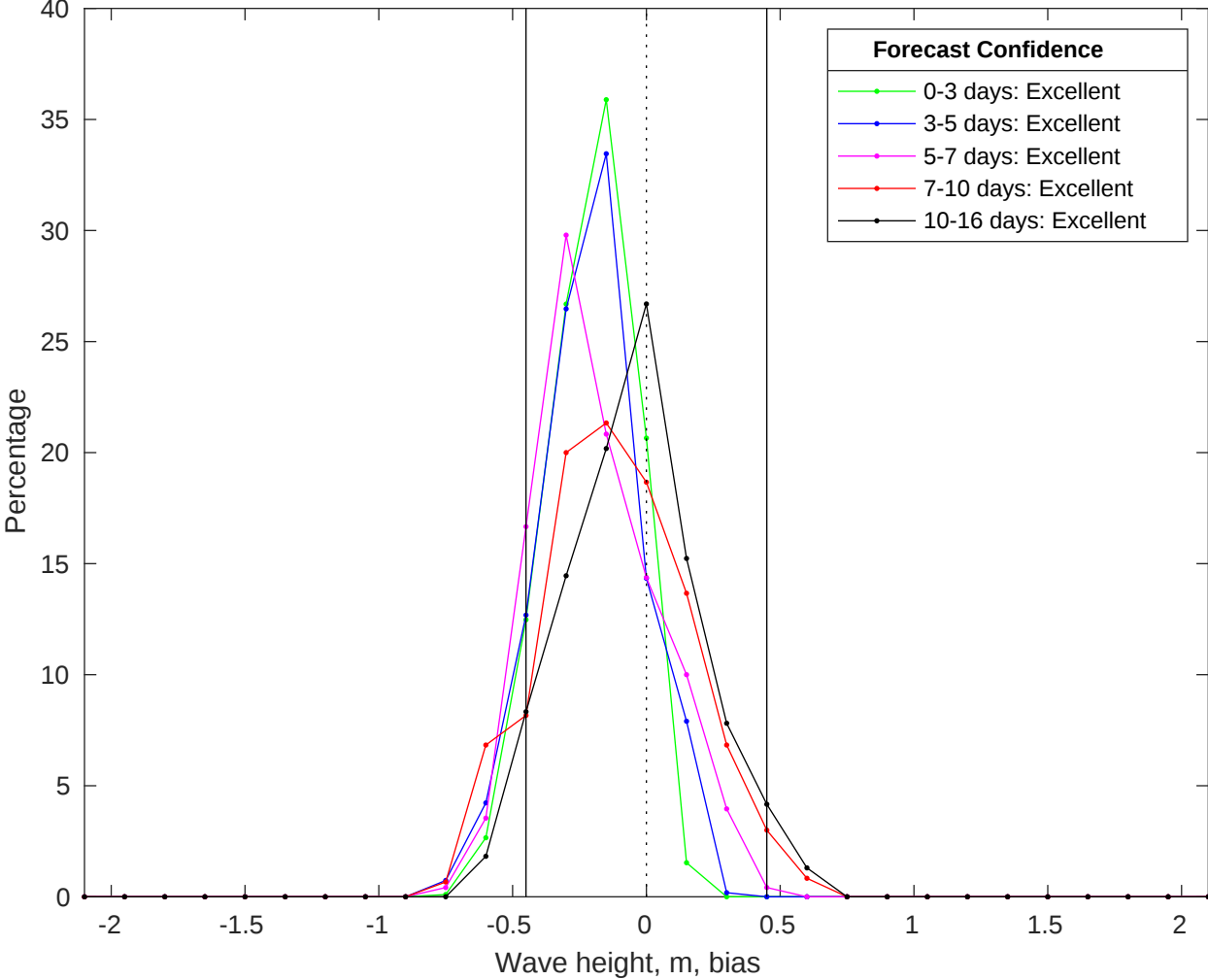
NDBC 41040 vs GFS Waves Bias Histogram: 12-Jul-2025
