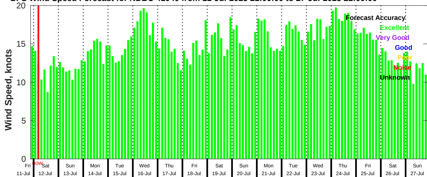
GFS Wind Speed Forecast for NDBC 41040 from 11-Jul-2025 21:00:00 to 27-Jul-2025 21:00:00
