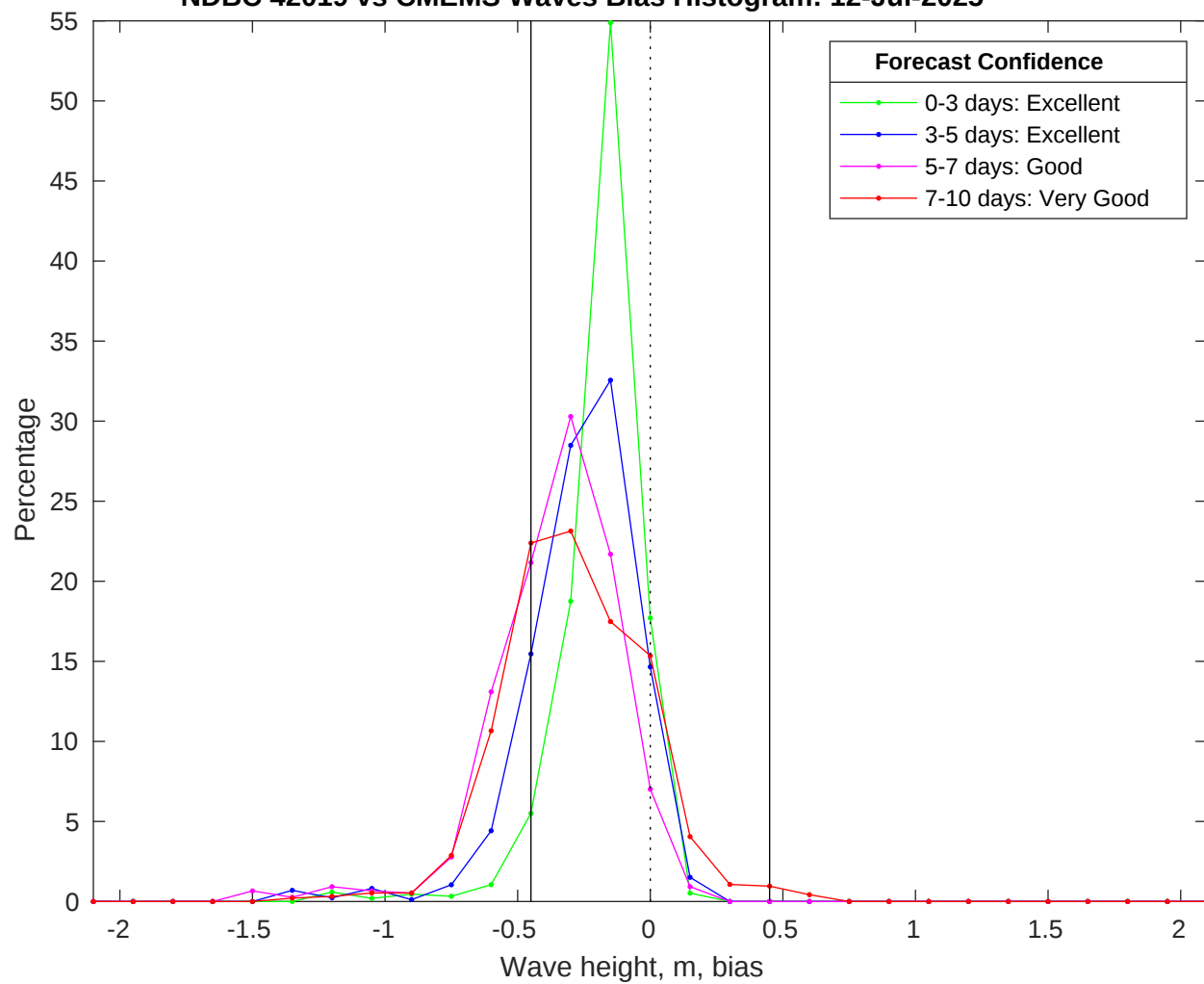
NDBC 42019 vs CMEMS Waves Bias Histogram: 12-Jul-2025
