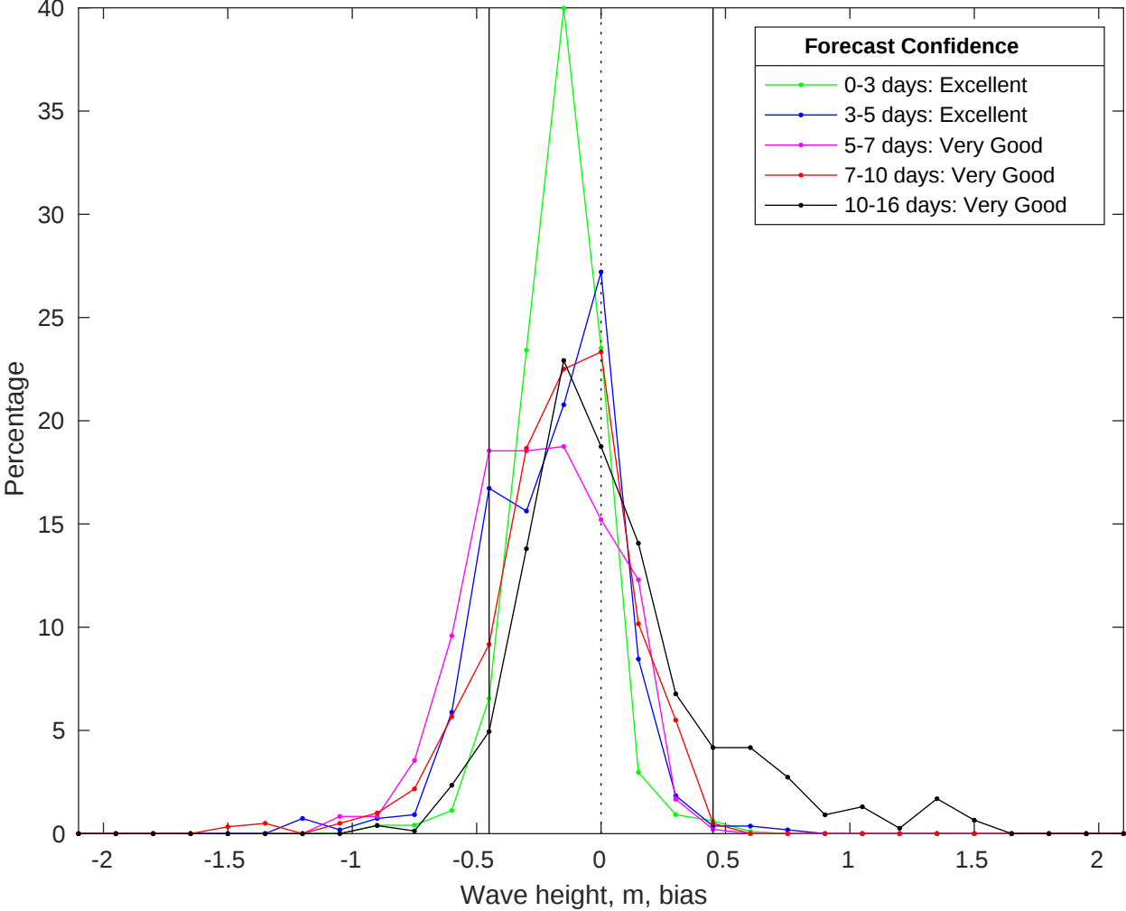
NDBC 42019 vs GFS Waves Bias Histogram: 12-Jul-2025
