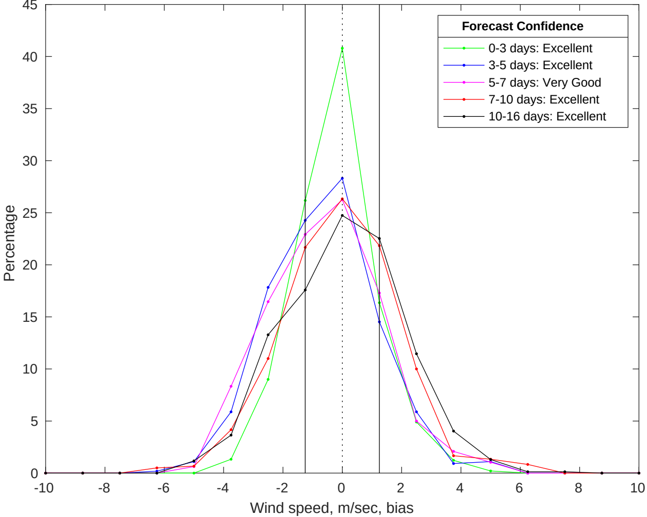
NDBC 42019 vs GFS Winds Bias Histogram: 12-Jul-2025
