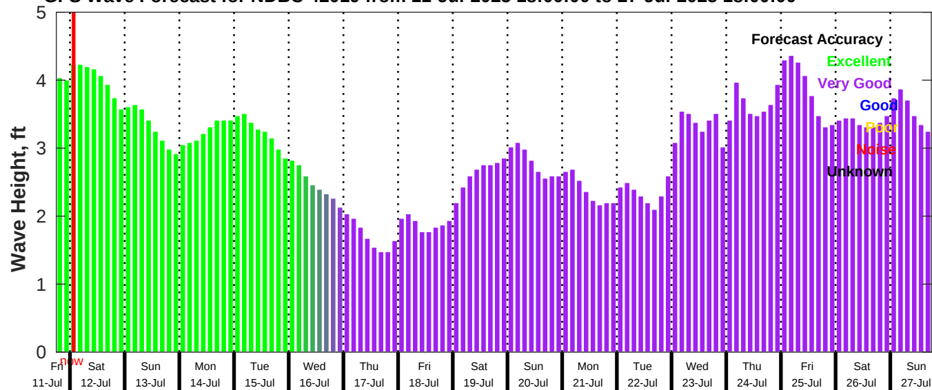
GFS Wave Forecast for NDBC 42019 from 11-Jul-2025 18:00:00 to 27-Jul-2025 18:00:00
