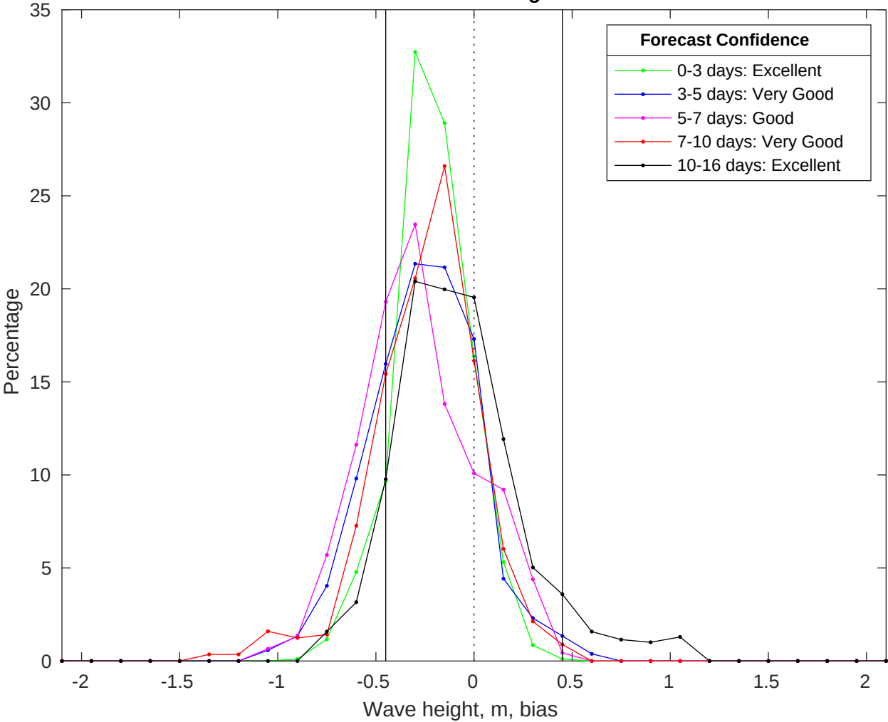
NDBC 42020 vs GFS Waves Bias Histogram: 11-Jul-2025
