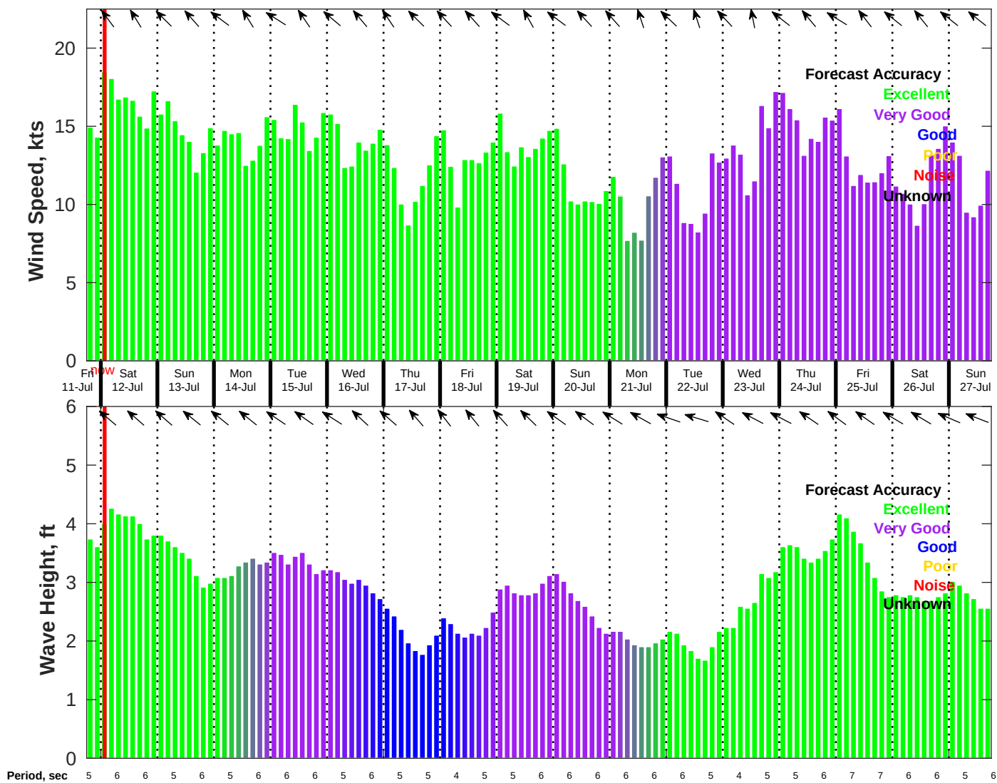
Wind & Wave Forecast for NDBC 42020 from 11-Jul-2025 18:00:00 to 27-Jul-2025 18:00:00
