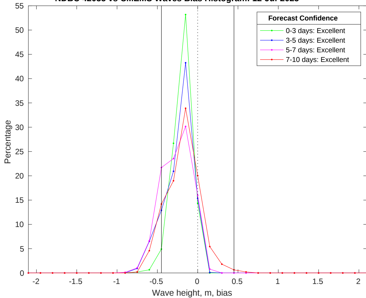
NDBC 42035 vs CMEMS Waves Bias Histogram: 12-Jul-2025
