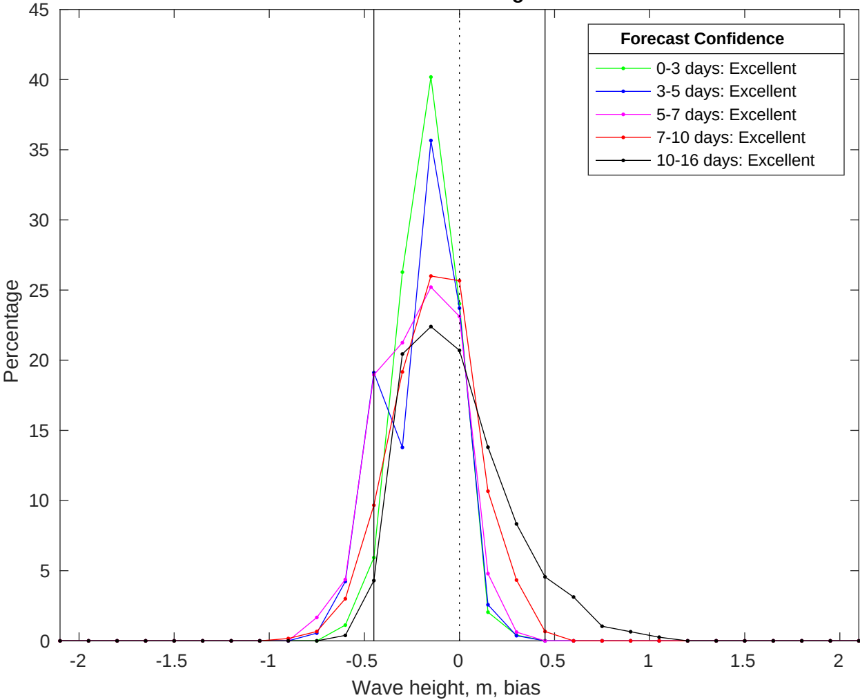
NDBC 42035 vs GFS Waves Bias Histogram: 12-Jul-2025
